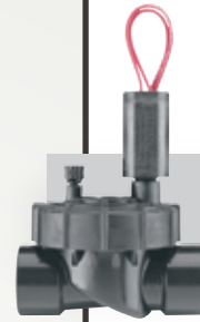
PGV-100JT - G: Inlet Diameter: 1" 5½" H x 4½" L x 3¼" W
