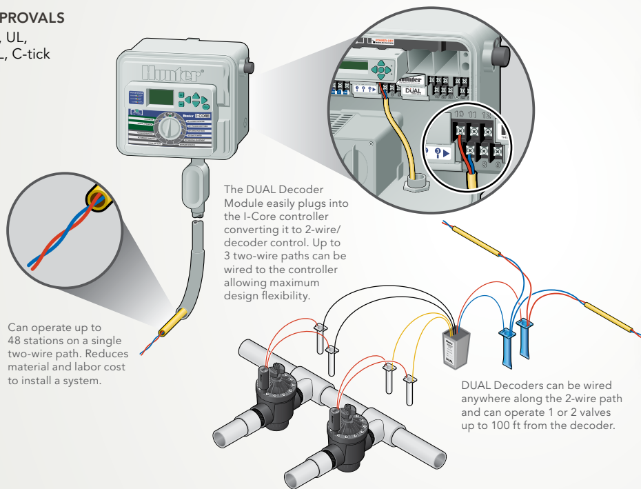
DUAL decoders and surge arrester: 3" H x 1 3/4" W x 2" D
